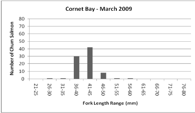
Figure 7A. Fork length frequency distribution of juvenile chum salmon captured at Cornet Bay sites in March, 2009.
