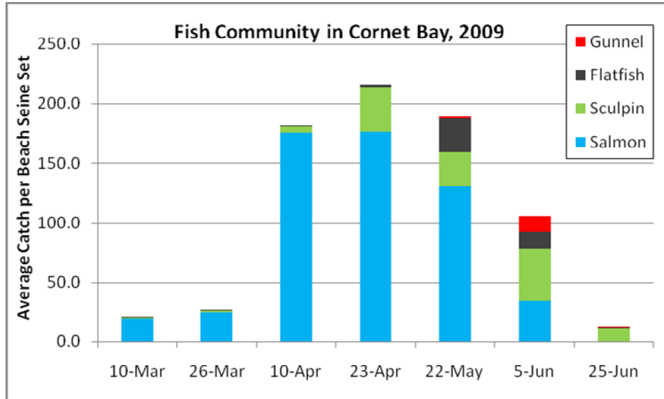
Figure 8. Fish Community and Relative Abundance in Cornet Bay, 2009.
