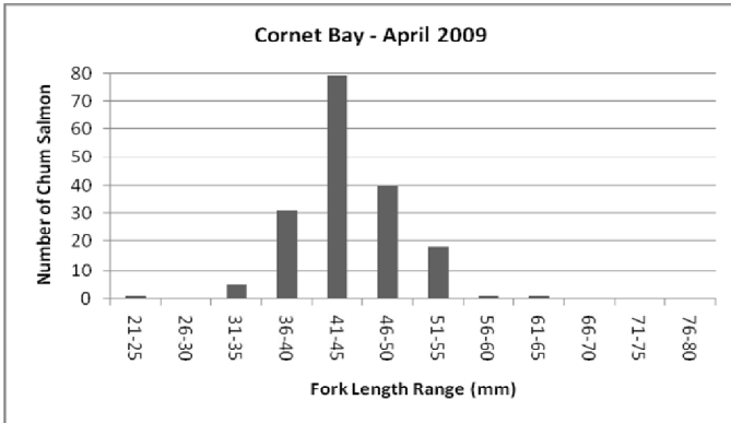
Figure 7B. Fork length frequency distribution of juvenile chum salmon captured at Cornet Bay sites in April, 2009.
