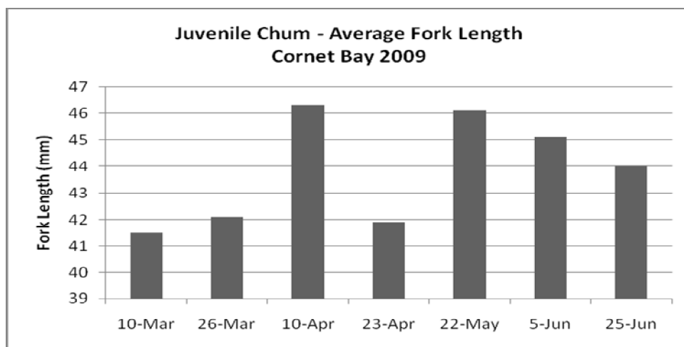
Figure 6. Average fork length of juvenile chum salmon caught at Cornet Bay, 2009.
