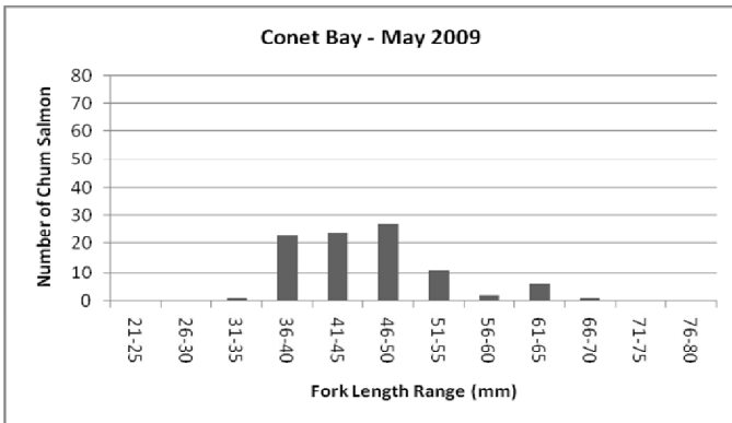
Figure 7C. Fork length frequency distribution of juvenile chum salmon captured at Cornet Bay sites in May, 2009.
