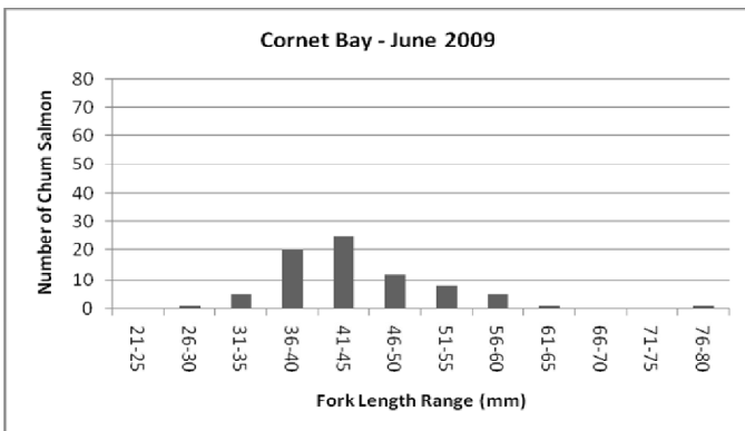
Figure 7D. Fork length frequency distribution of juvenile chum salmon captured at Cornet Bay sites in June, 2009.
