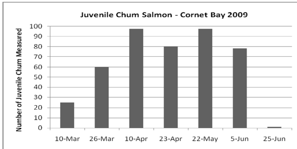
Figure 5. Number of Juvenile Chum Measured at Cornet Bay, 2009.
